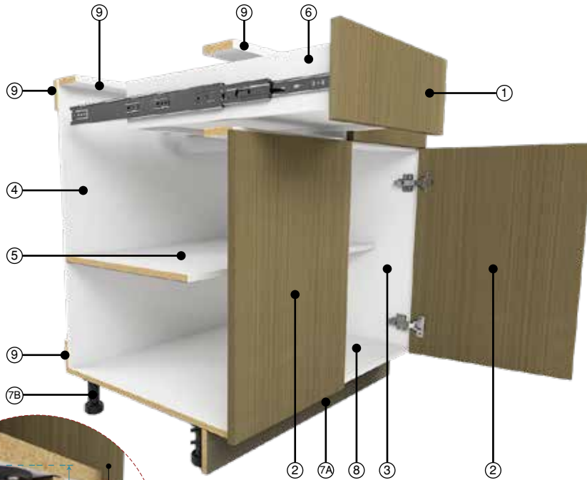
7B) Adjustable Plastic Leg a. front of cabinet b. toe board
