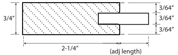
Straight Shaker Door Profile
