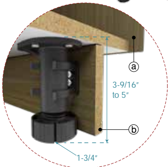
7B) Adjustable Plastic Leg a. front of cabinet b. toe board
