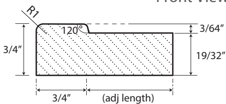
Slim Shaker Door Front View
